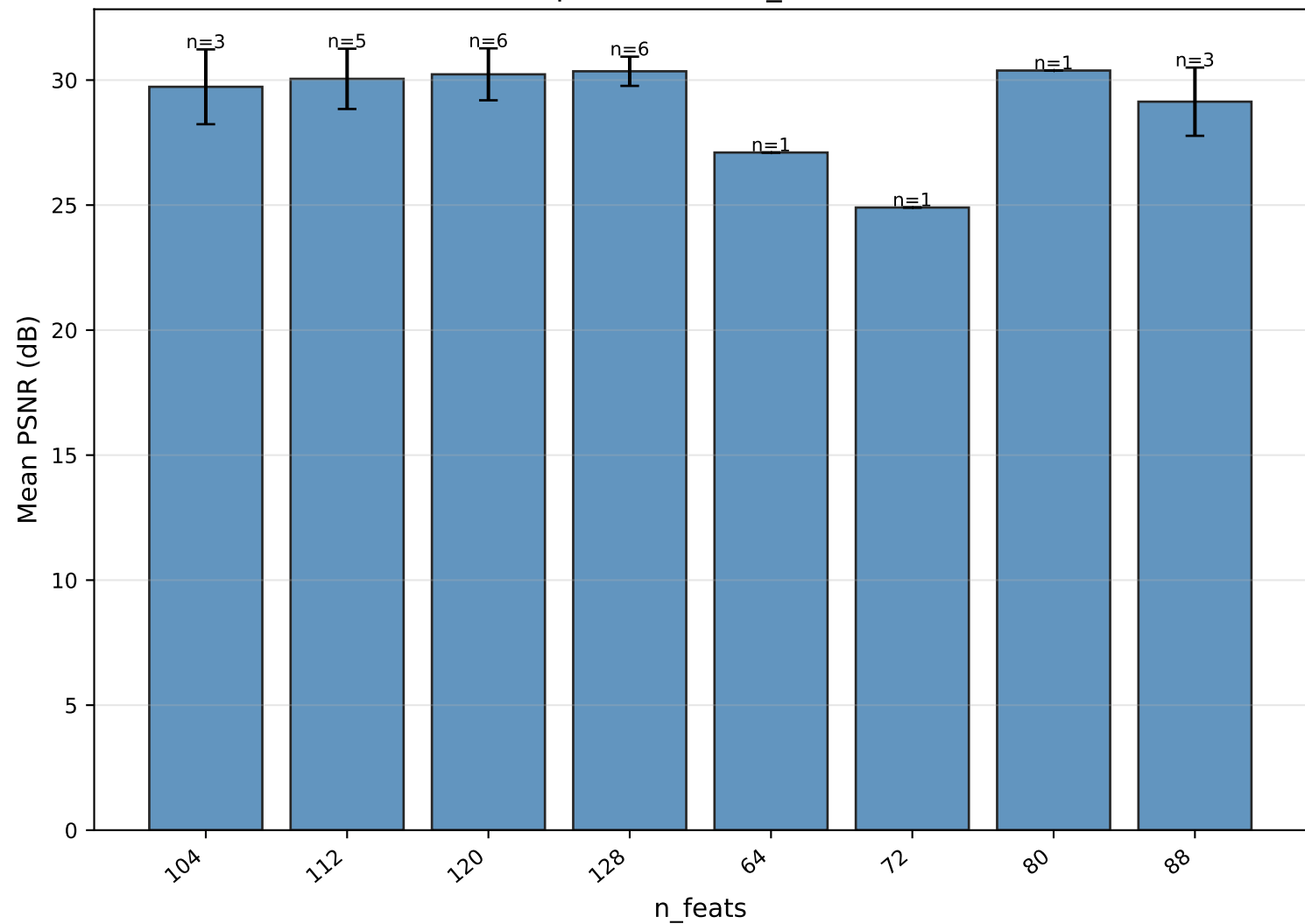
Mean PSNR per value of n_feats — OmniSR
